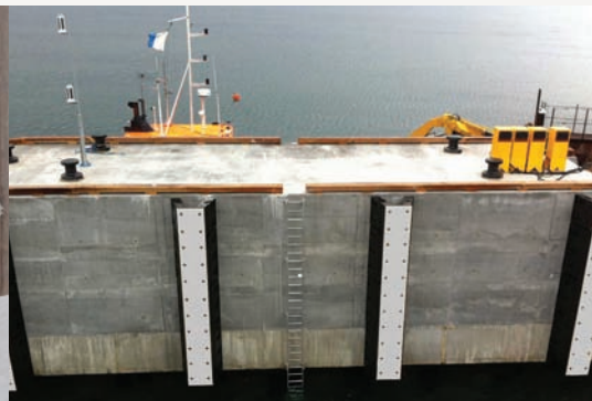
King Hy-Pact® | Dock Fenders
